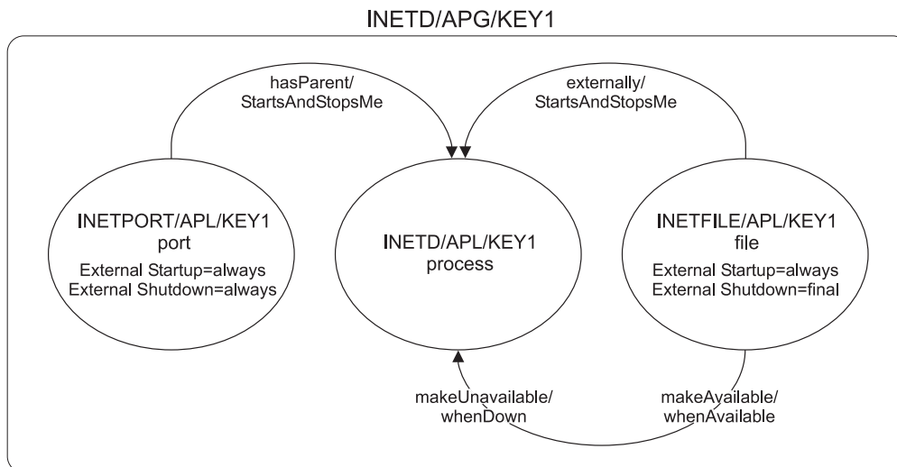
Figure 14. Dependency Graphic for inetd
