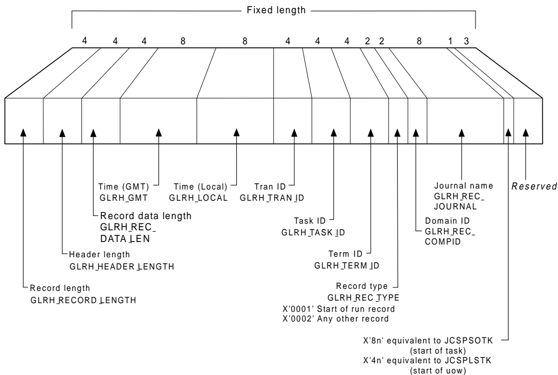
Figure 57. Format of a general log record header
