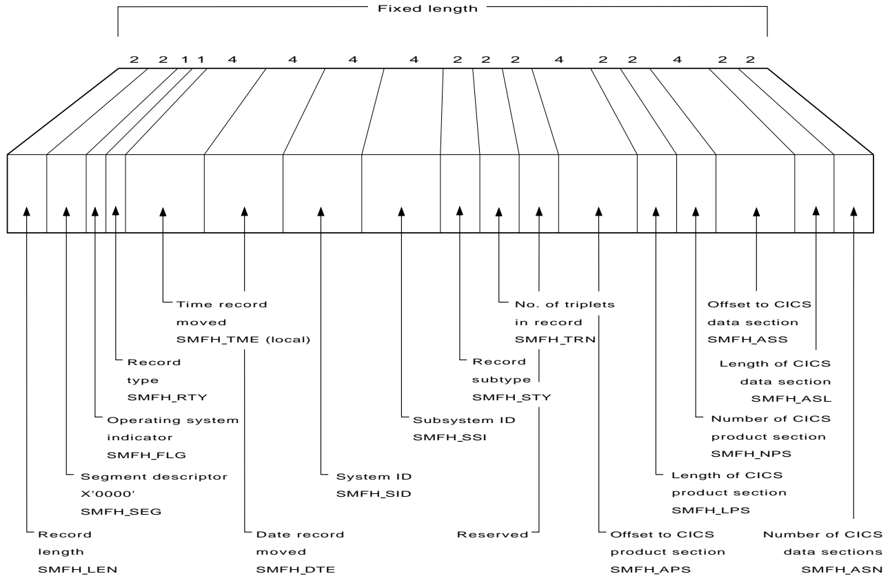
Figure 82. Format of the SMF block header
