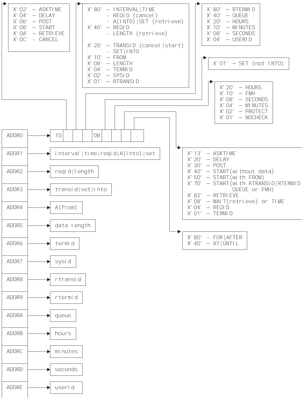
Figure 1. The command-level parameter structure for interval control
