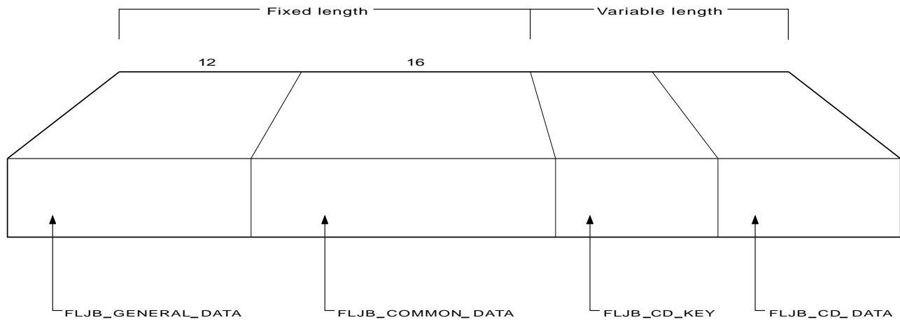
Figure 60. Layout of record written for read-only, read-update, write-update, write-add, and write-add-complete record types
