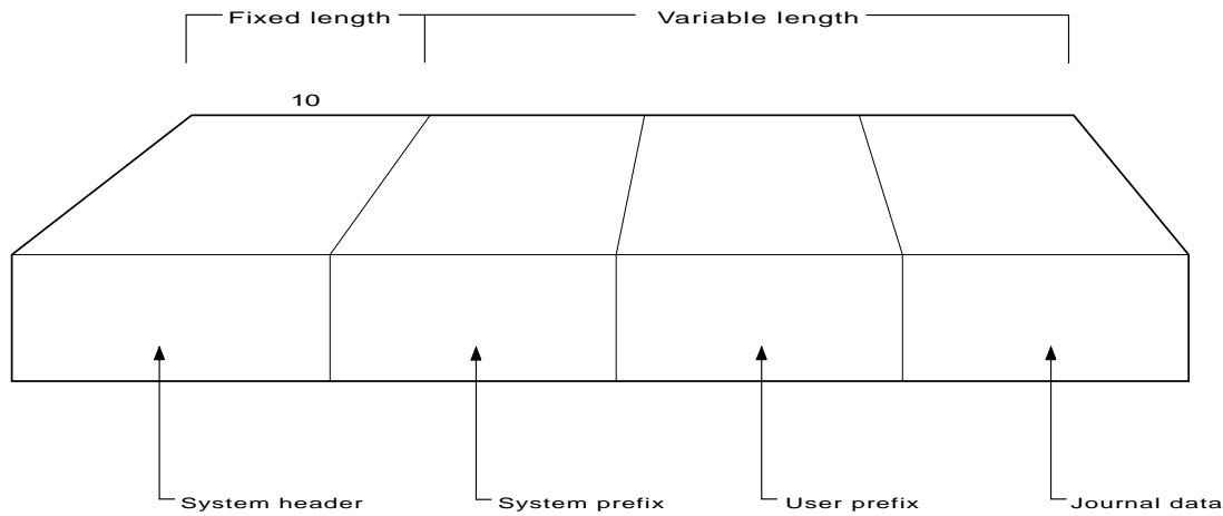
Figure 75. Format of COMPAT41 journal record
