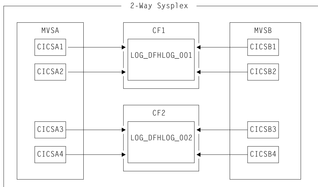
Figure 8. Sharing system logger structures between MVS images
