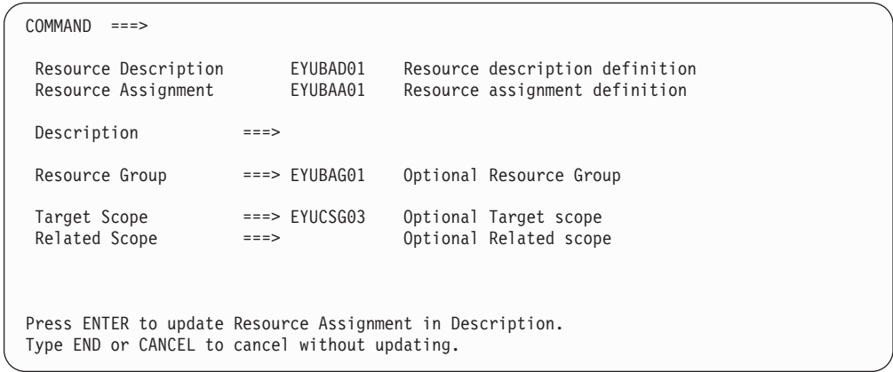
Figure 111. Updating the association between a resource description and assignment
