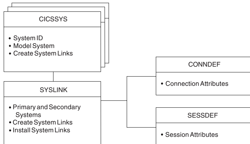
Figure 6. Views for defining links between CICS systems
