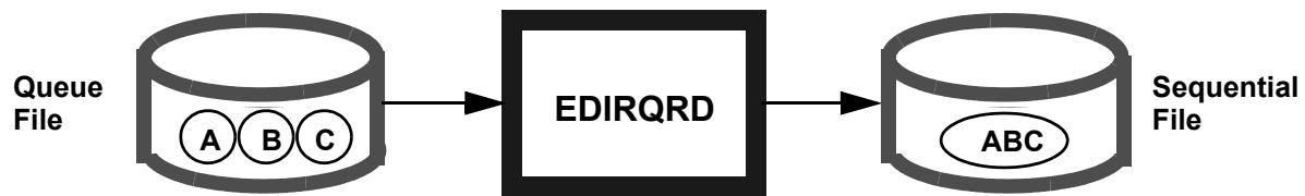
Figure 1.7 Document Group/Unit of Work Batch Read
