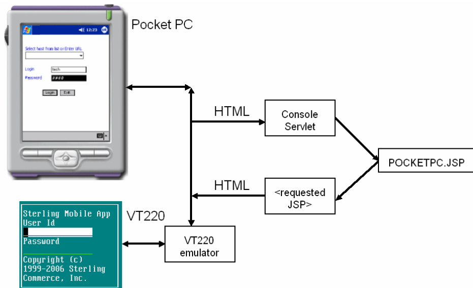
Figure 2–2 Mobile Architecture
