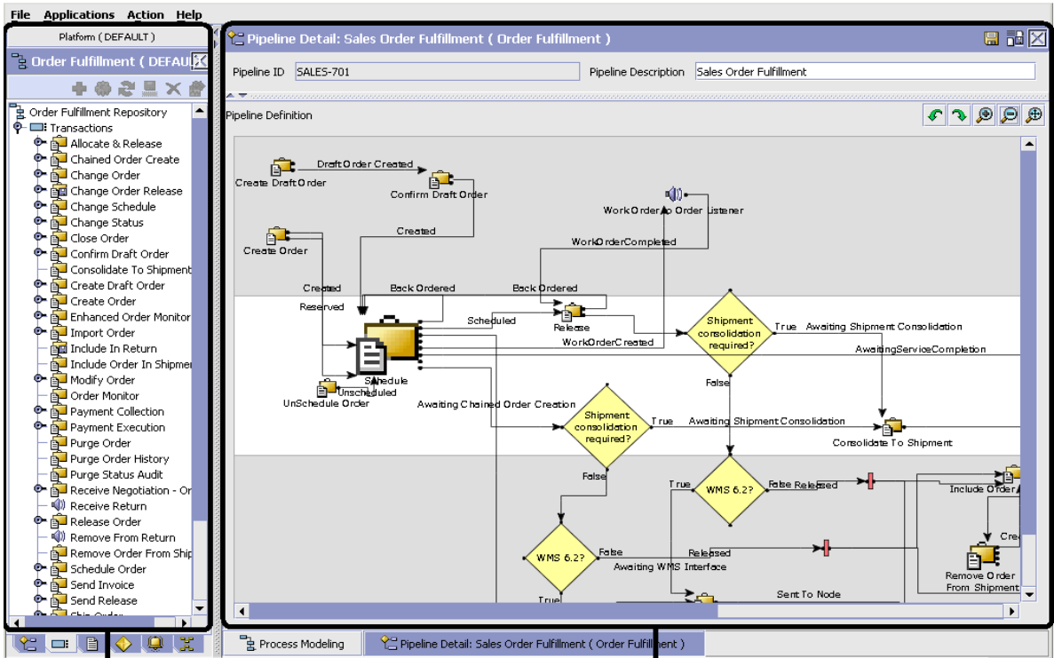
Figure 2–11 Drag and Drop Window Example
