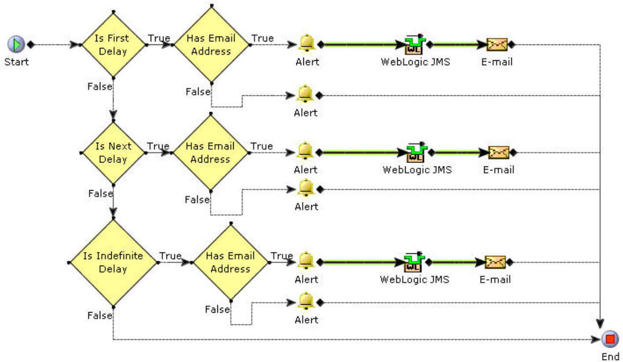
Figure 7. YCD_FTC_SEND_NOTIFICATION Service
