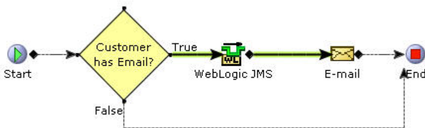
Figure 9. YCD_ShipmentNotificationEmail_1.0 service
