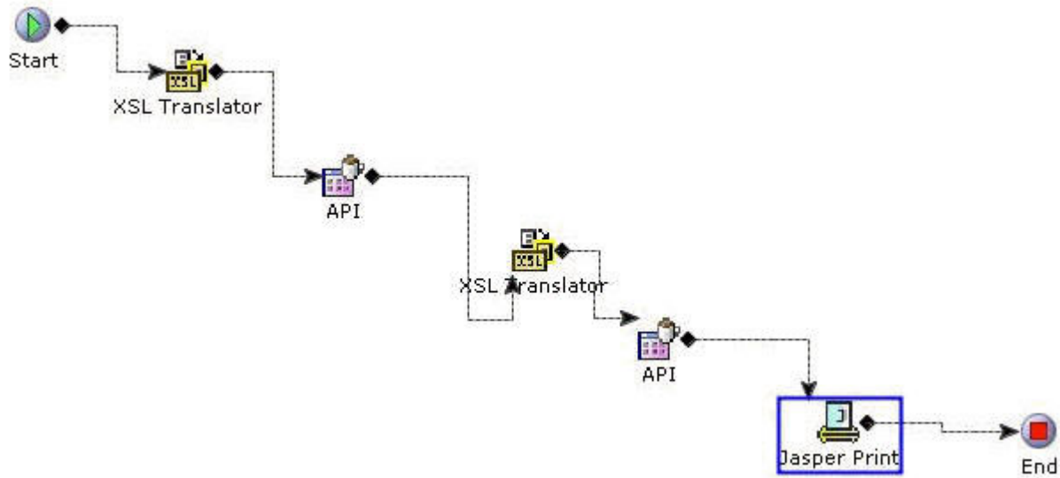
Figure 19. YCD_PrintOrderSummary_3.0 service
