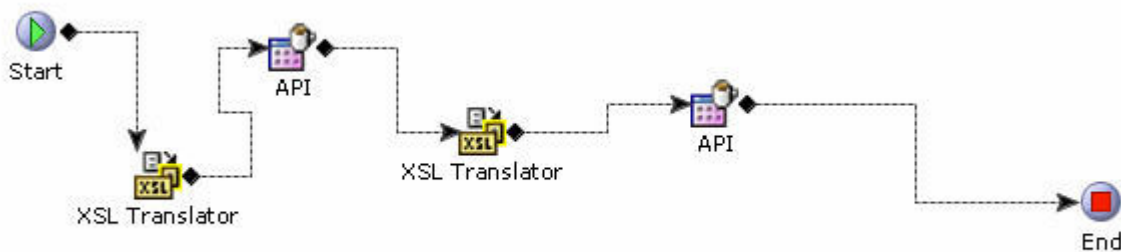
Figure 22. YCD_Change_Status_Backroom_Pick_8.0 service
