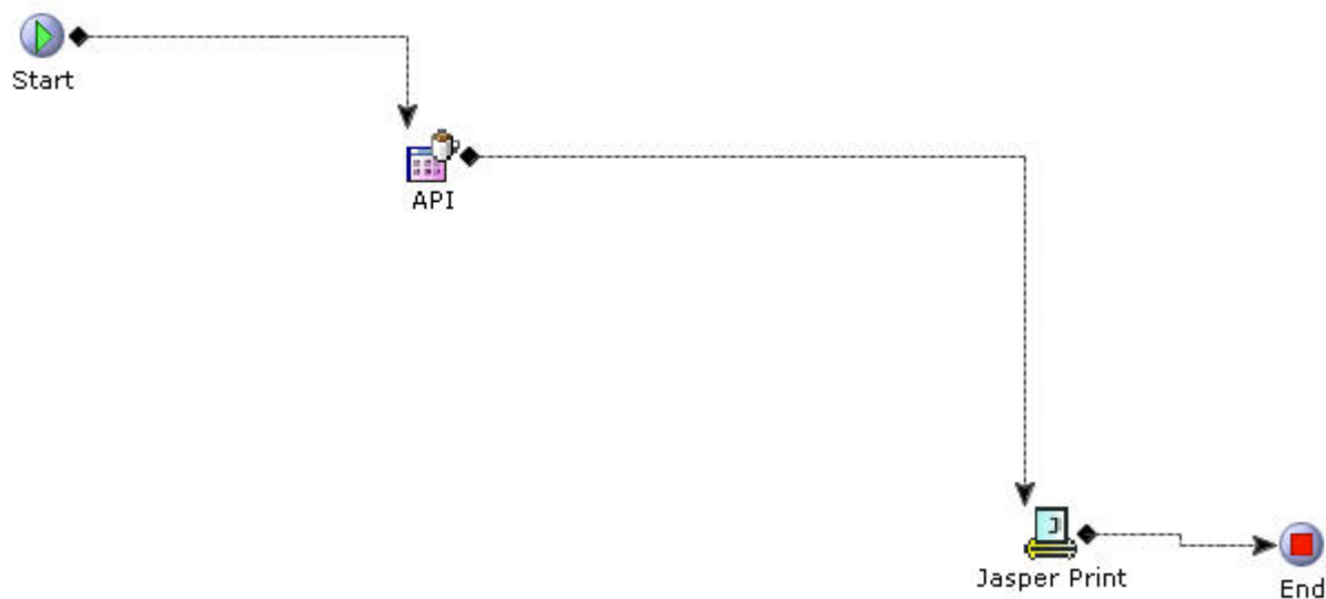
Figure 20. YCD_PrintChangeOrderSummaryPrintReport_3.0
