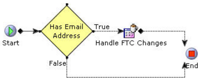
Figure 6. YCD_FTC_DELAY_EMAIL, YCD_FTC_FIRST_DELAY_EMAIL, and YCD_FTC_INDEFINITE_DELAY_EMAIL Services
