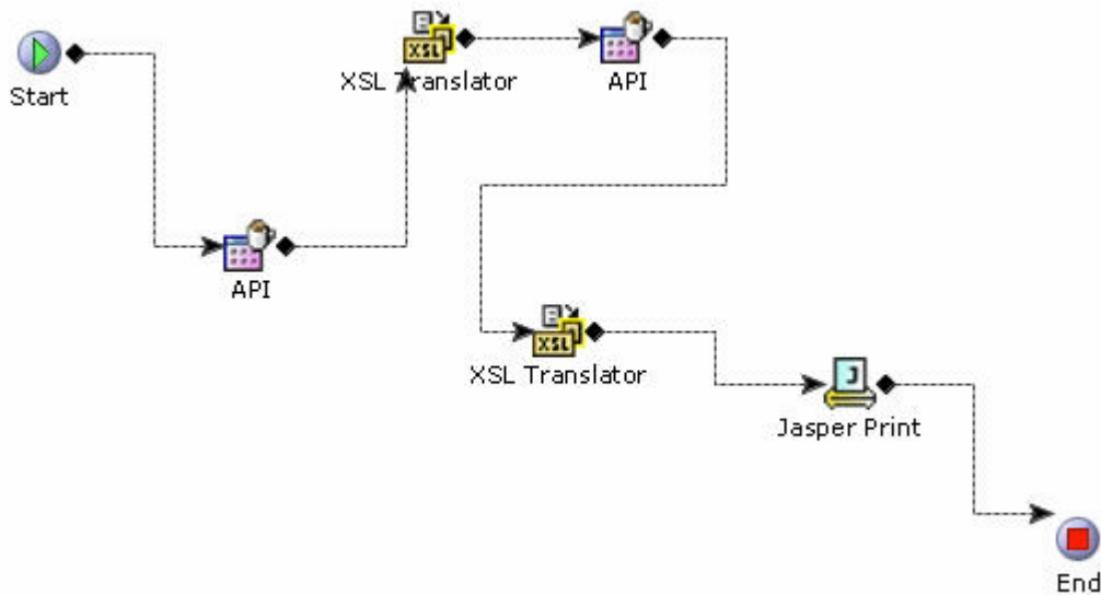
Figure 21. YCD_PrintPickTicket_8.0 service
