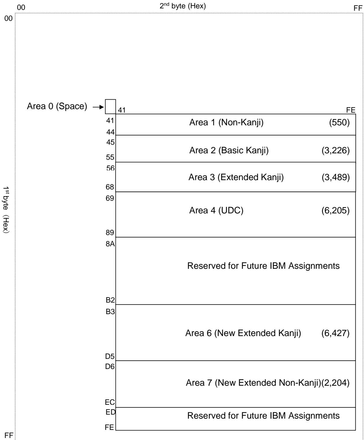
Figure 1. Code Structure for Japanese DBCS-Host (Overview)
