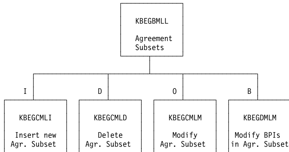
Figure 121. Local Administration, option set structure overview. I , D , O , and B are action codes on the panel.
