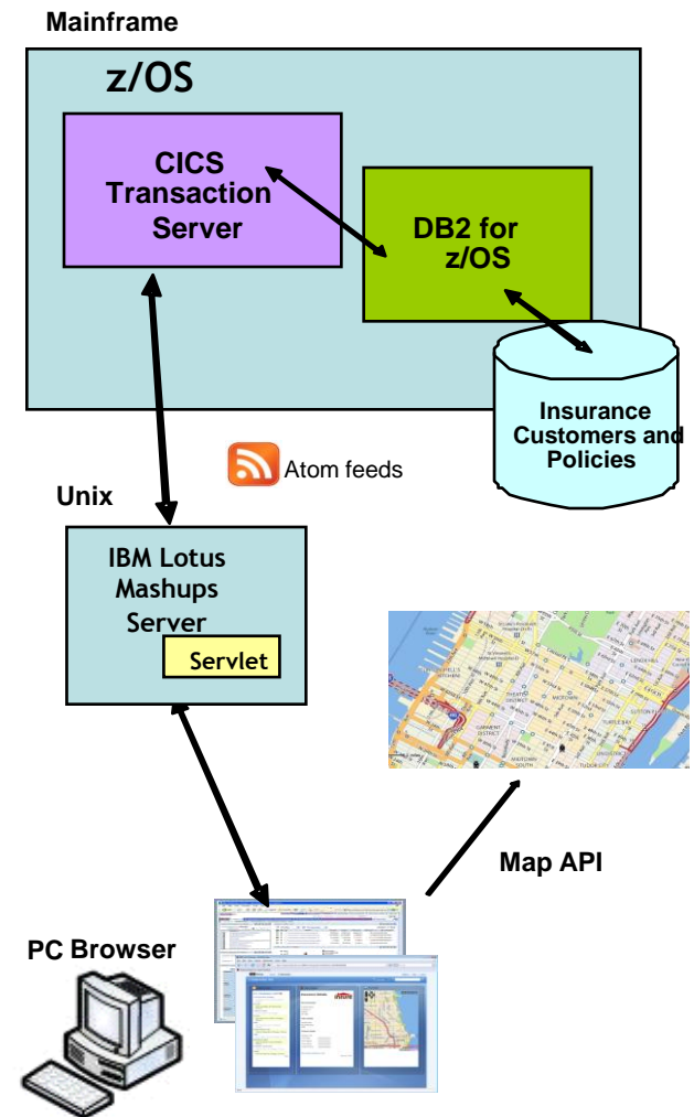
High level architecture: CICS Atom feeds
