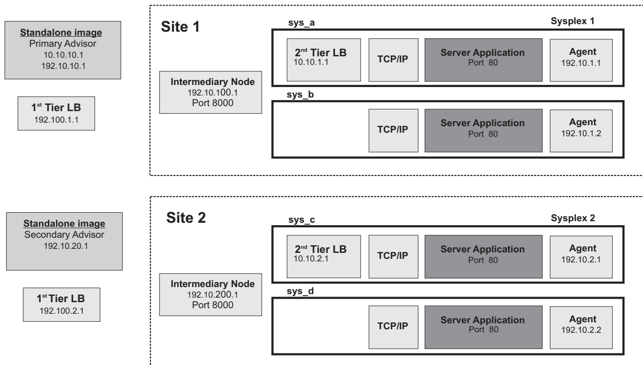
Figure 14. Multi-site Workload Lifeline configuration Example 2
