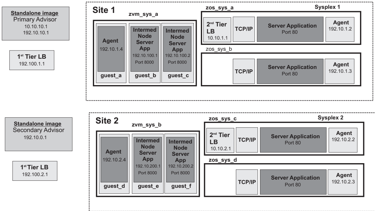
Figure 23. Multi-site Workload Lifeline configuration Example 5
