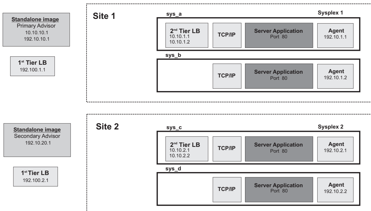
Figure 17. Multi-site Workload Lifeline configuration Example 3
