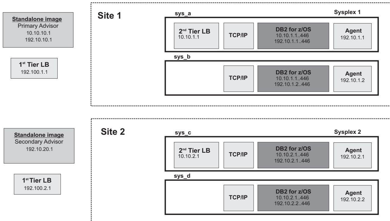
Figure 29. Multi-site Workload Lifeline configuration Example 7
