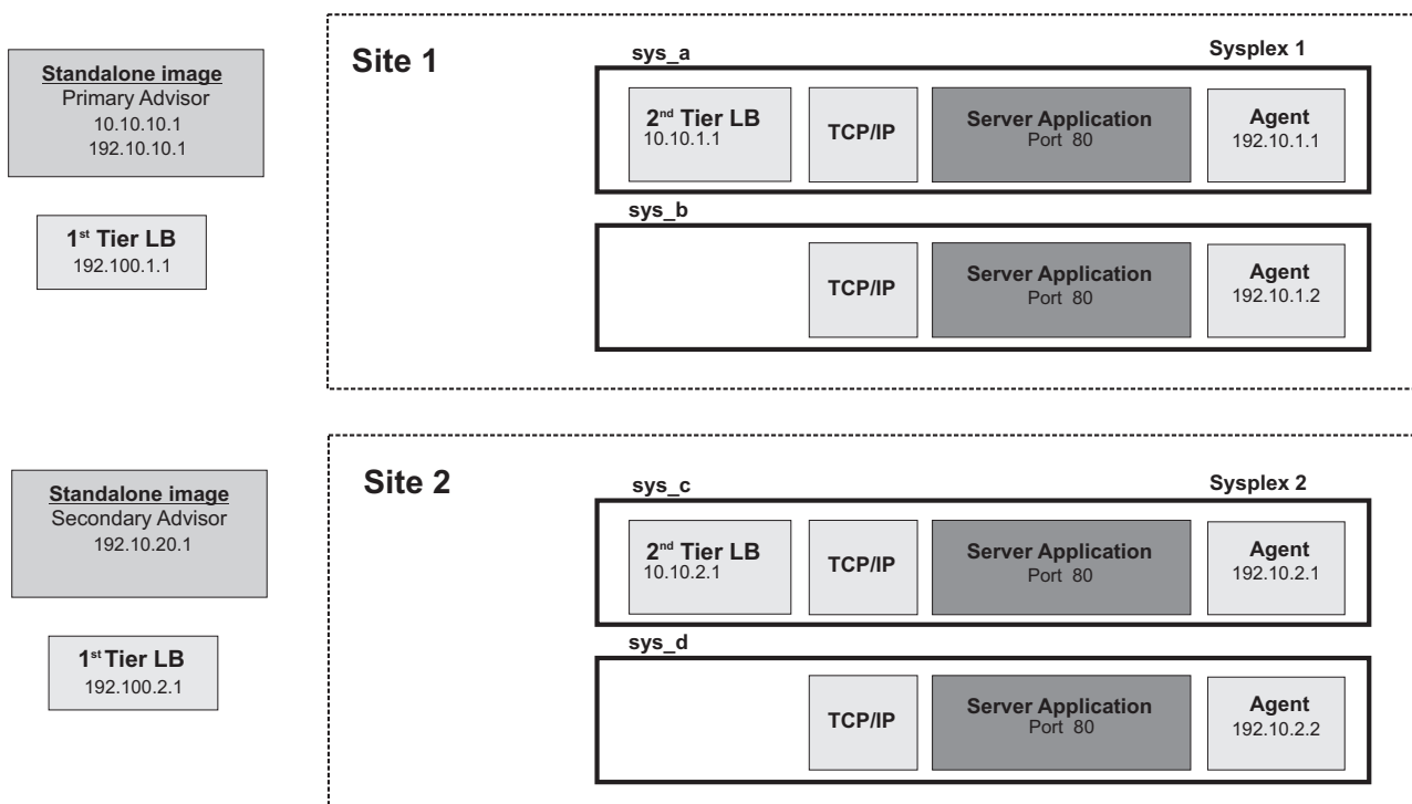
Figure 11. Multi-site Workload Lifeline configuration Example 1
