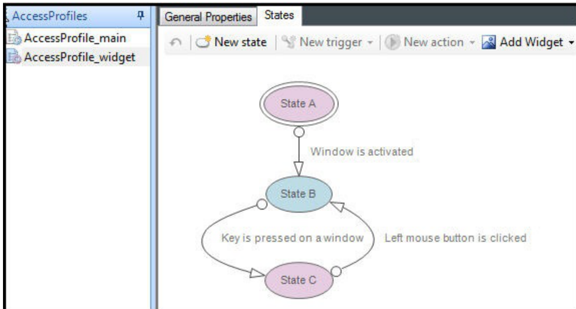
Figure 1. Sample AccessProfile widget
