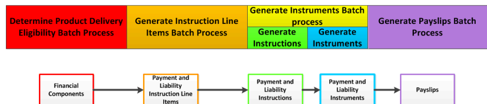
Figure 3.1 The Financial Batch Suite
