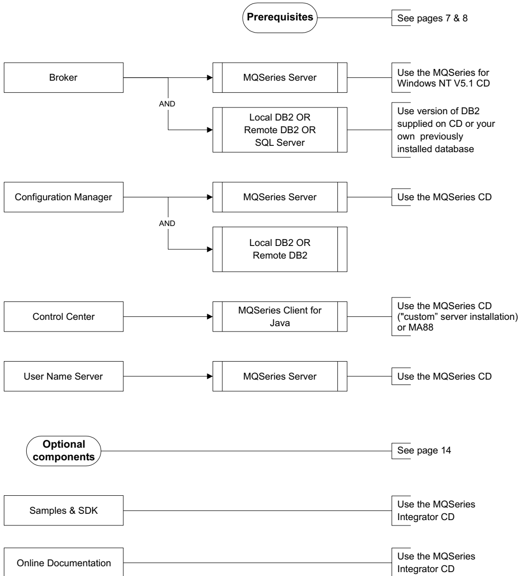
Figure 1. Summary of product prerequisite
