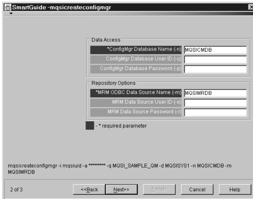
Figure 3. Create Configuration Manager: screen 2
