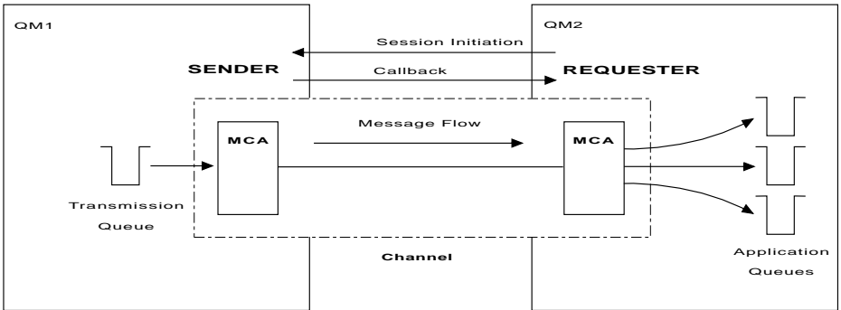
Figure 8. A requester-sender channel
