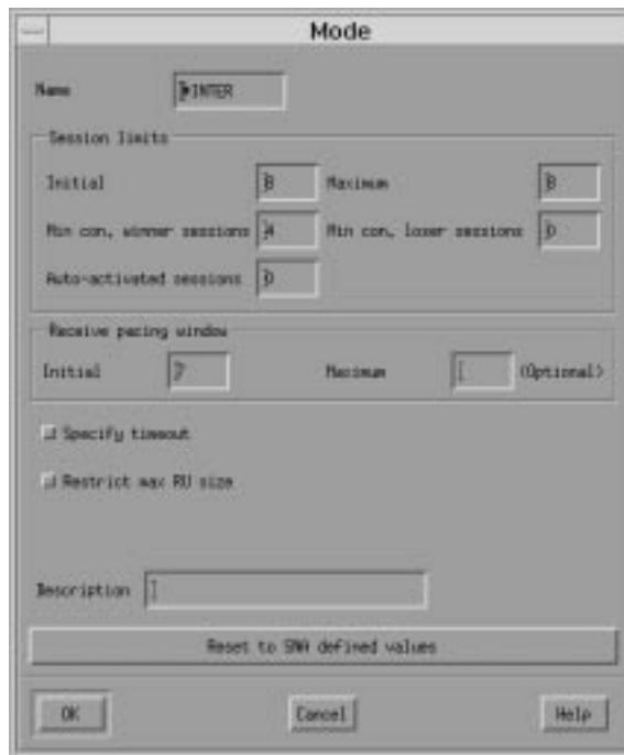
Figure 34. Mode window
