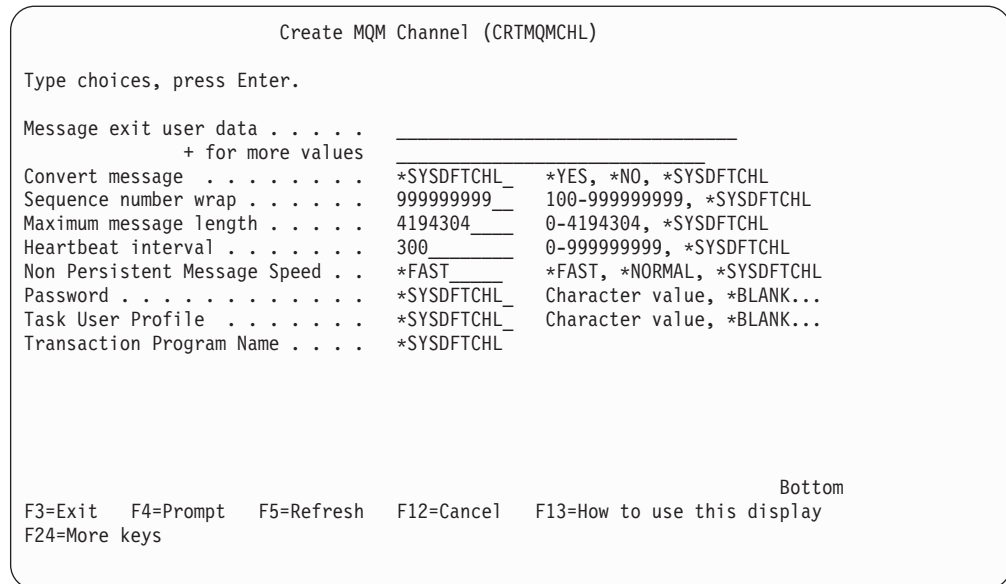
Figure 95. Create channel (4)
