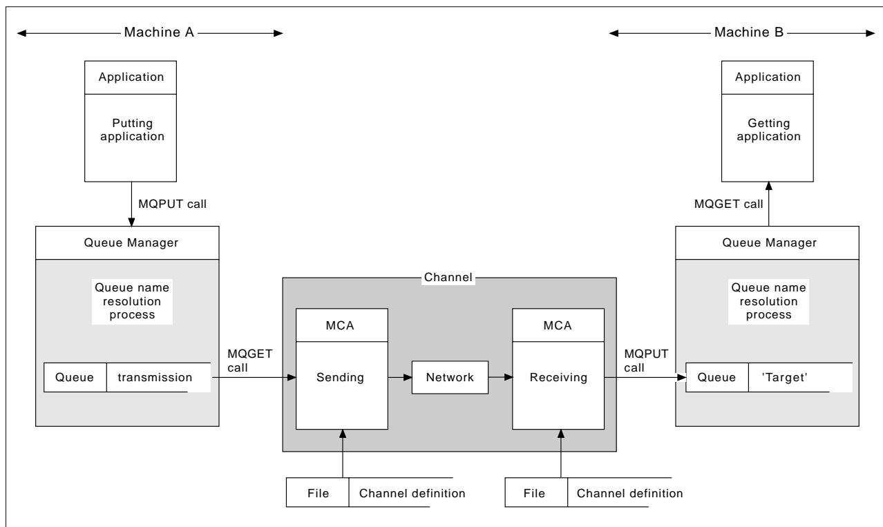
Figure 144. Name resolution
