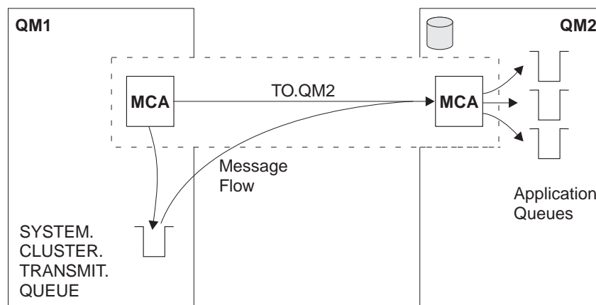
Figure 6. A cluster-sender channel
