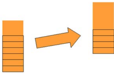
Figure 4: Messaging technology
