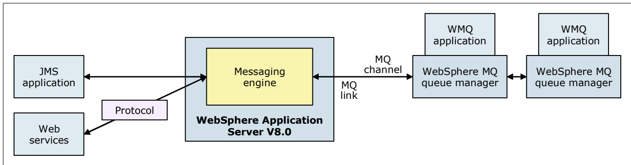
Figure 22 WebSphere Application Server integration with WebSphere MQ
