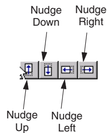
Figure 63. Nudge toolbar
