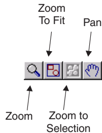
Figure 64. Zoom/Pan toolbar
