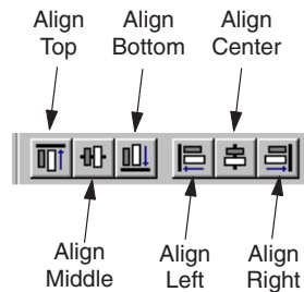
Figure 57. Alignment toolbar
