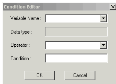
Figure 38. Condition Editor
