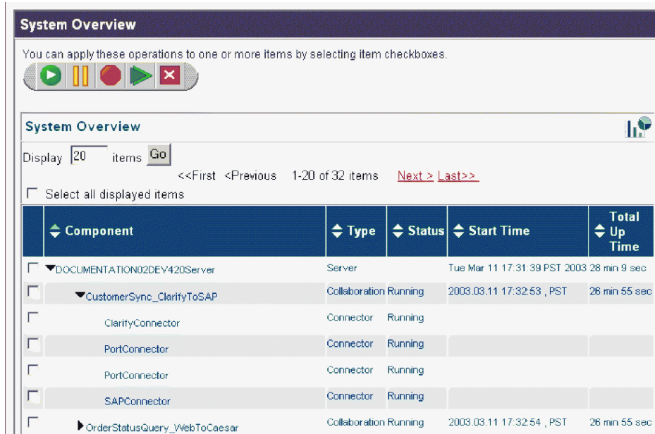
Figure 24. System Monitor, System Overview displaying connector state
