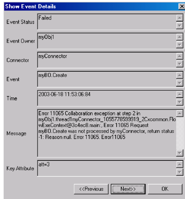
Figure 70. Flow Manager Show Event Details dialog box
