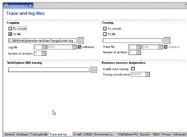
Figure 50. Edit Configuration tool, Trace/Log Files tab
