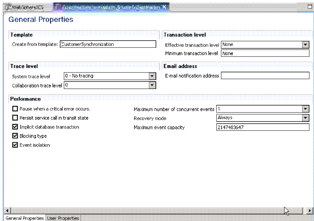
Figure 30. Properties dialog box, Collaboration General Properties tab
