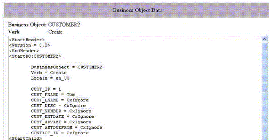
Figure 64. Failed Event Manager Business Object Data dialog box
