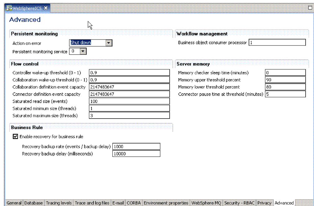
Figure 23. Edit configuration tool, Advanced tab
