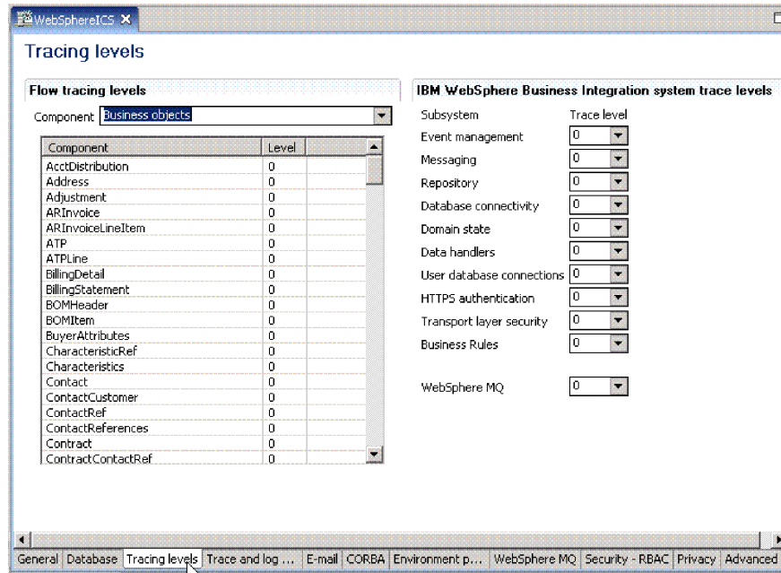
Figure 51. Edit Configuration tool, Tracing Levels tab
