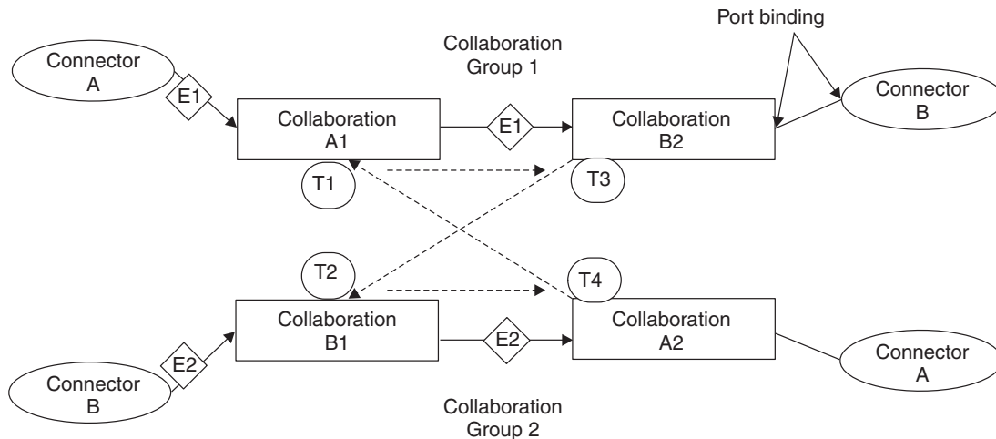
Figure 72. Deadlock between collaboration groups
