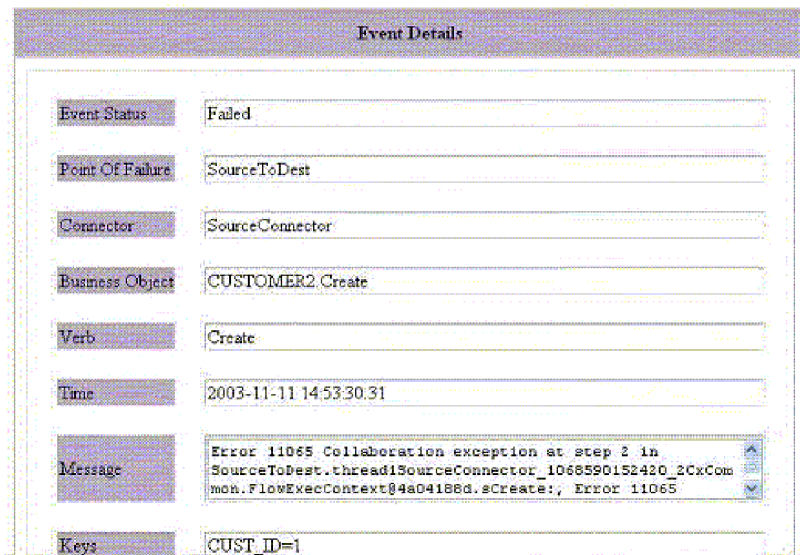
Figure 63. Failed Event Manager Event Details dialog box
