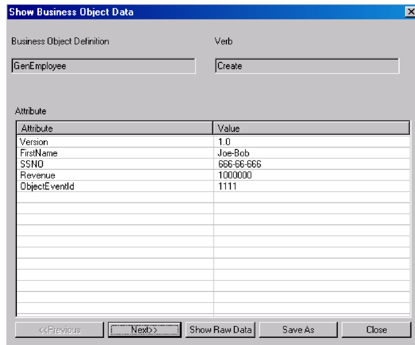
Figure 71. Show Business Object Data dialog box
