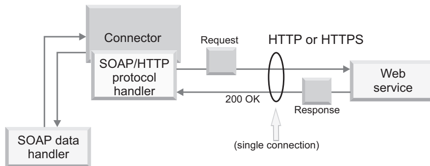
Figure 29. SOAP/HTTP-HTTPS protocol handler: asynchronous request processing
