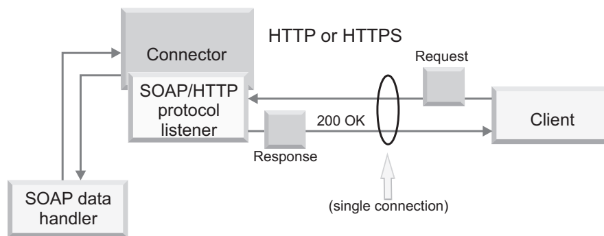
Figure 24. SOAP/HTTP protocol listener: synchronous event processing
