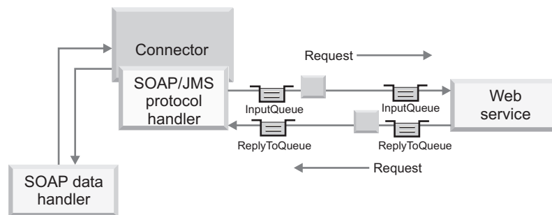
Figure 30. SOAP/JMS protocol handler: synchronous request processing
