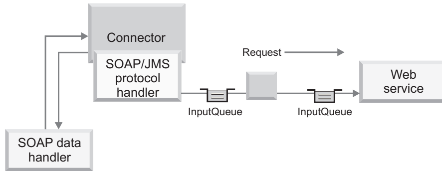
Figure 31. SOAP/JMS protocol handler: asynchronous request processing
