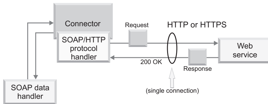
Figure 28. SOAP/HTTP-HTTPS protocol handler: synchronous request processing
