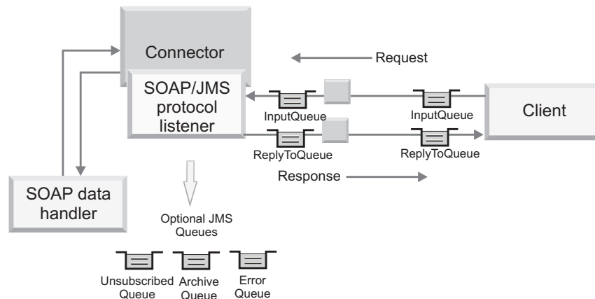
Figure 26. SOAP/JMS protocol listener: synchronous event processing
