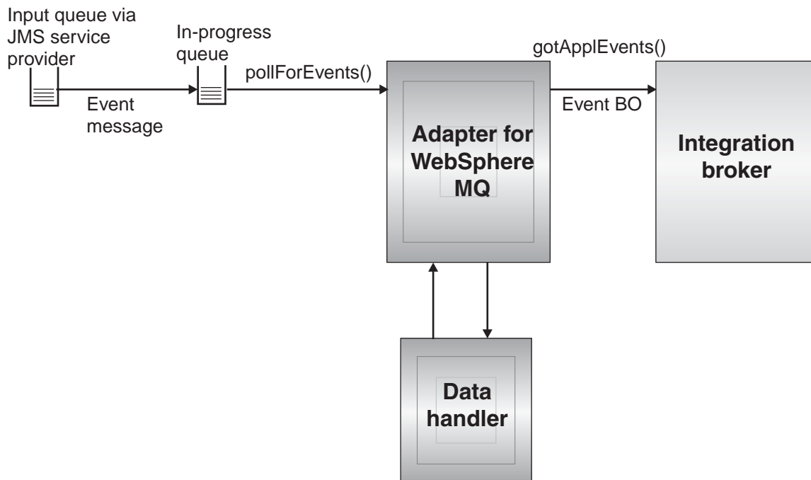
Figure 2. Application-connector communication method: Event delivery
