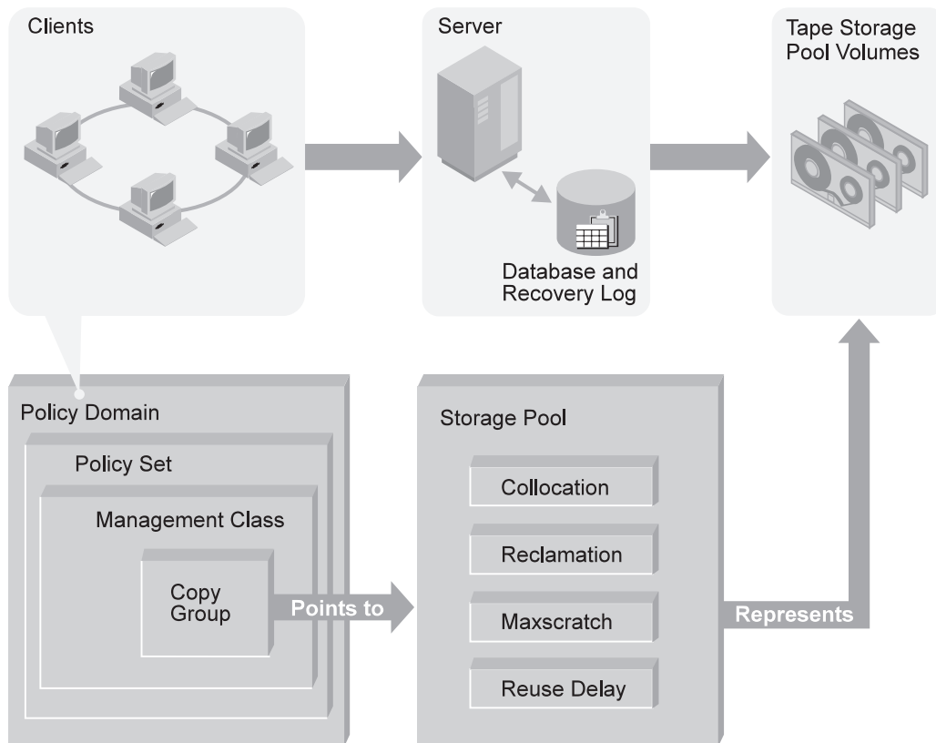
Figure 10. Using ADSM to Manage Media
