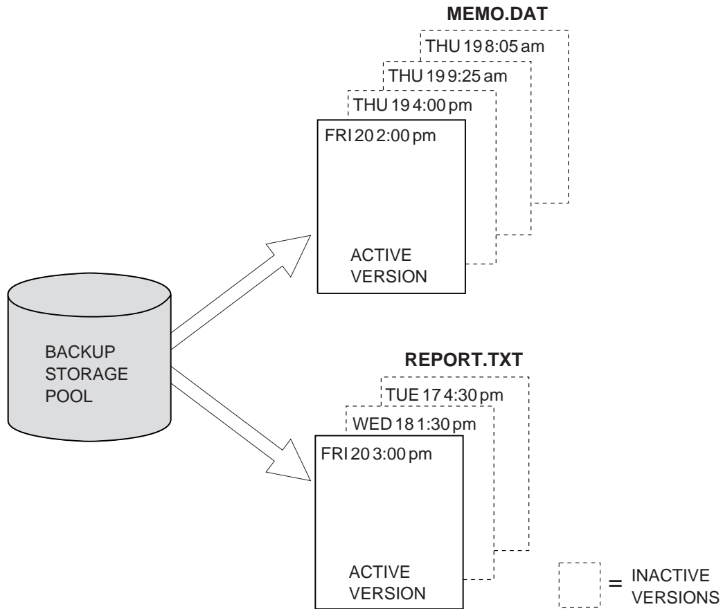
Figure 42. Example of Active and Inactive Versions of Backed Up Files
