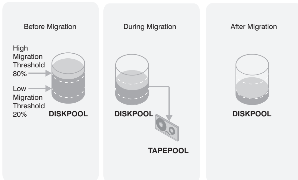
Figure 19. The Migration Process and Migration Thresholds
