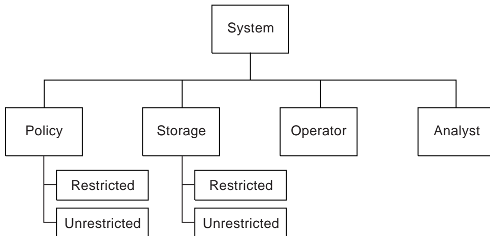
Figure 54. Administrative Privilege Classes
