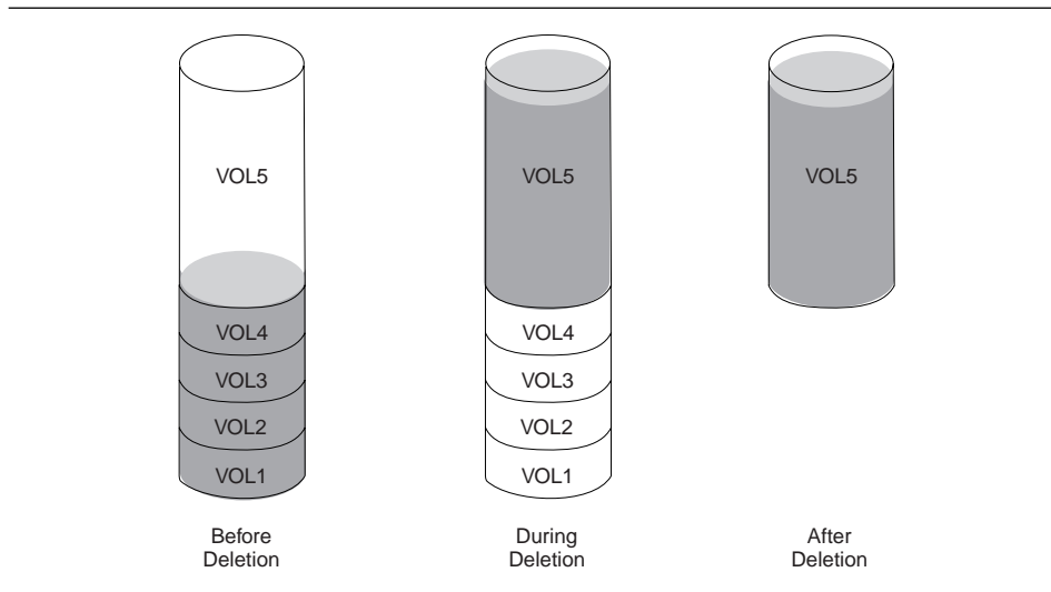
Figure 53. Deleting Database Volumes
