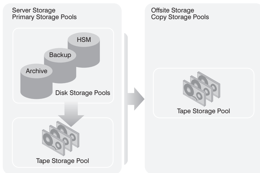
Figure 59. Copy Storage Pools
