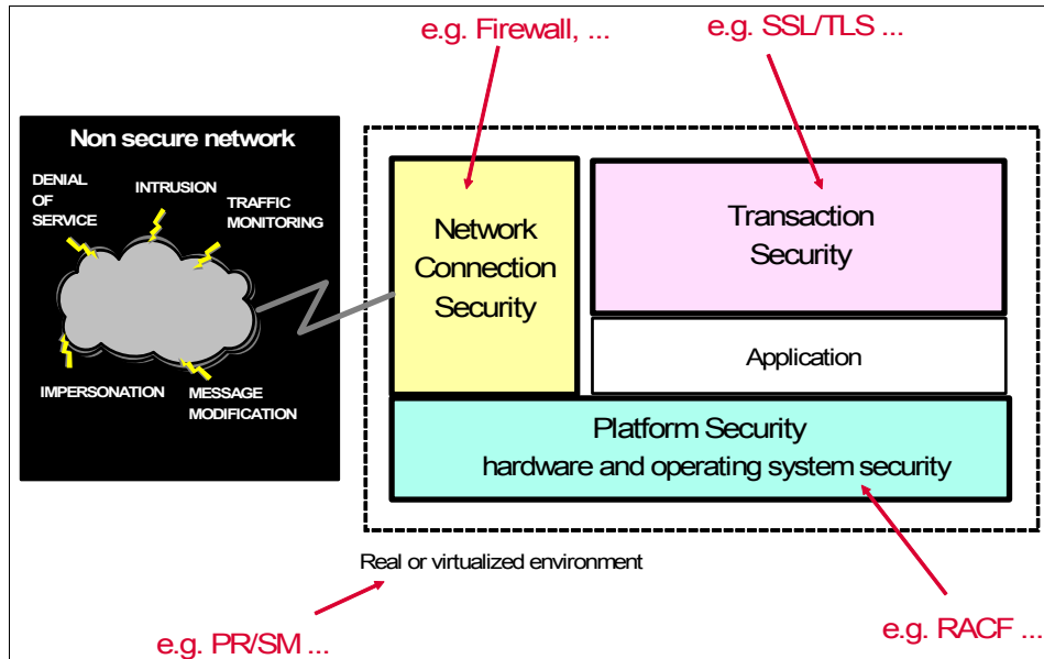
Figure 8-1 Network threats
