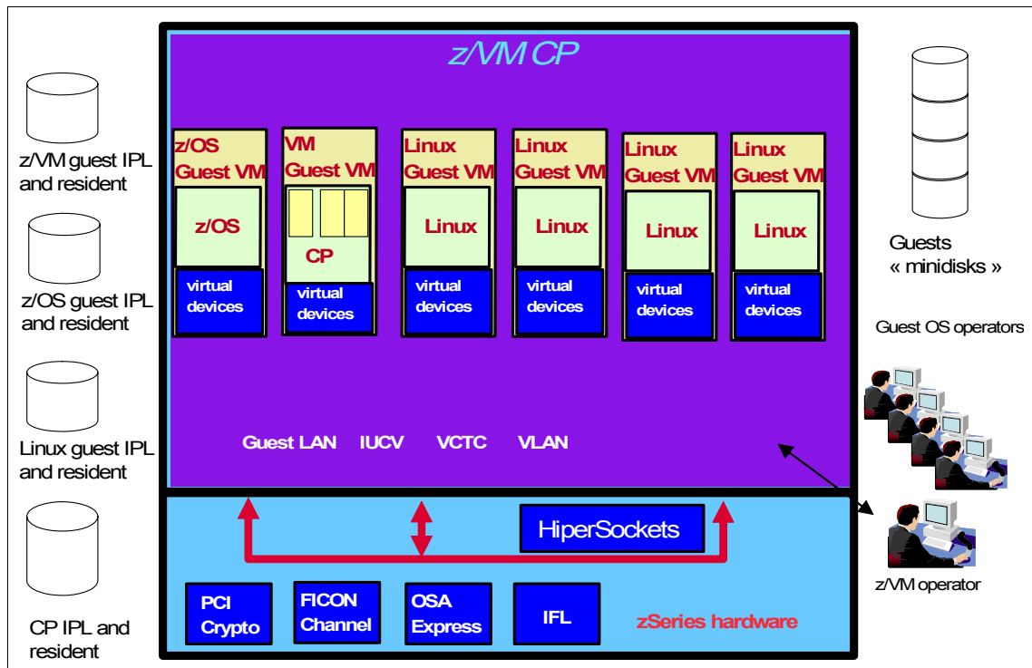
Figure 6-3 z/VM implementation
